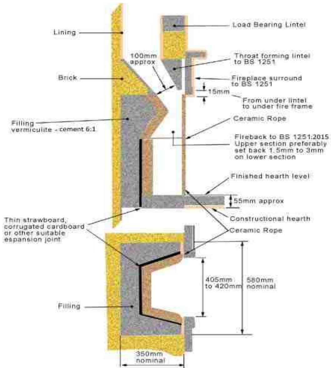
Fig 1. Setting for 400mm nominal inset open fire
